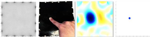
Figure 5. EIT technique based tracking workflow: Finite Element Model (Left), a 20 \times 20 cm sensor, the reconstructed image, and tracking through blob detection (Right).
