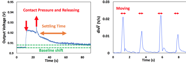
Figure 1. Voltage reading from a sensing channel fed with fixed DC current upon pressure (Left). Movement detection using \text{div}\bar{V}_i smoothed by a 5-frame running average (Right).
